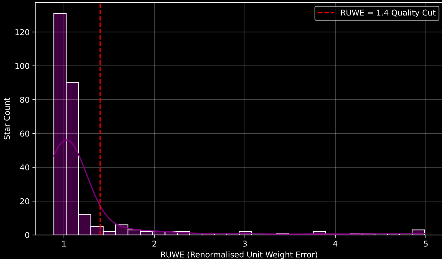
GALAH DR4 Field [1599] RUWE Distribution (n= 270)
