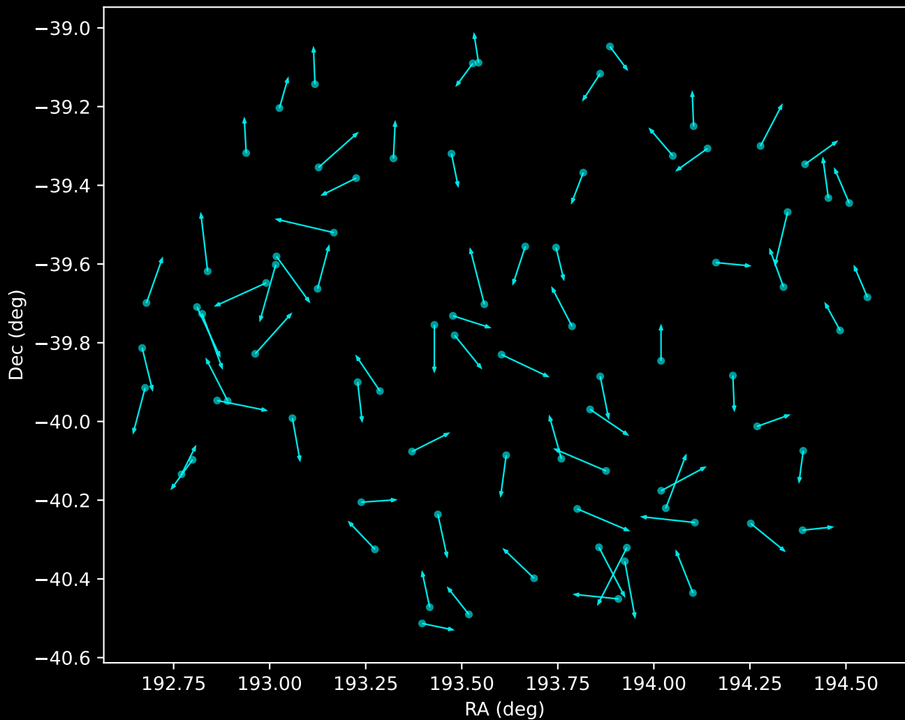
GALAH DR4 Noise Stream Proper Motion Vectors (n=79)
