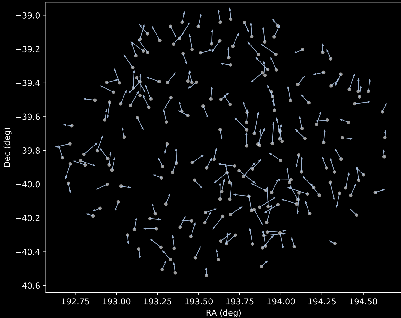
GALAH DR4 Cluster 1 Proper Motion Vectors (n=202)
