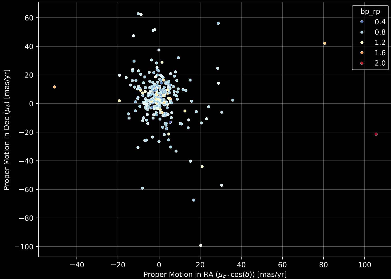
GALAH DR4 Field: [1599] Proper Motion Diagram (n= 286)
