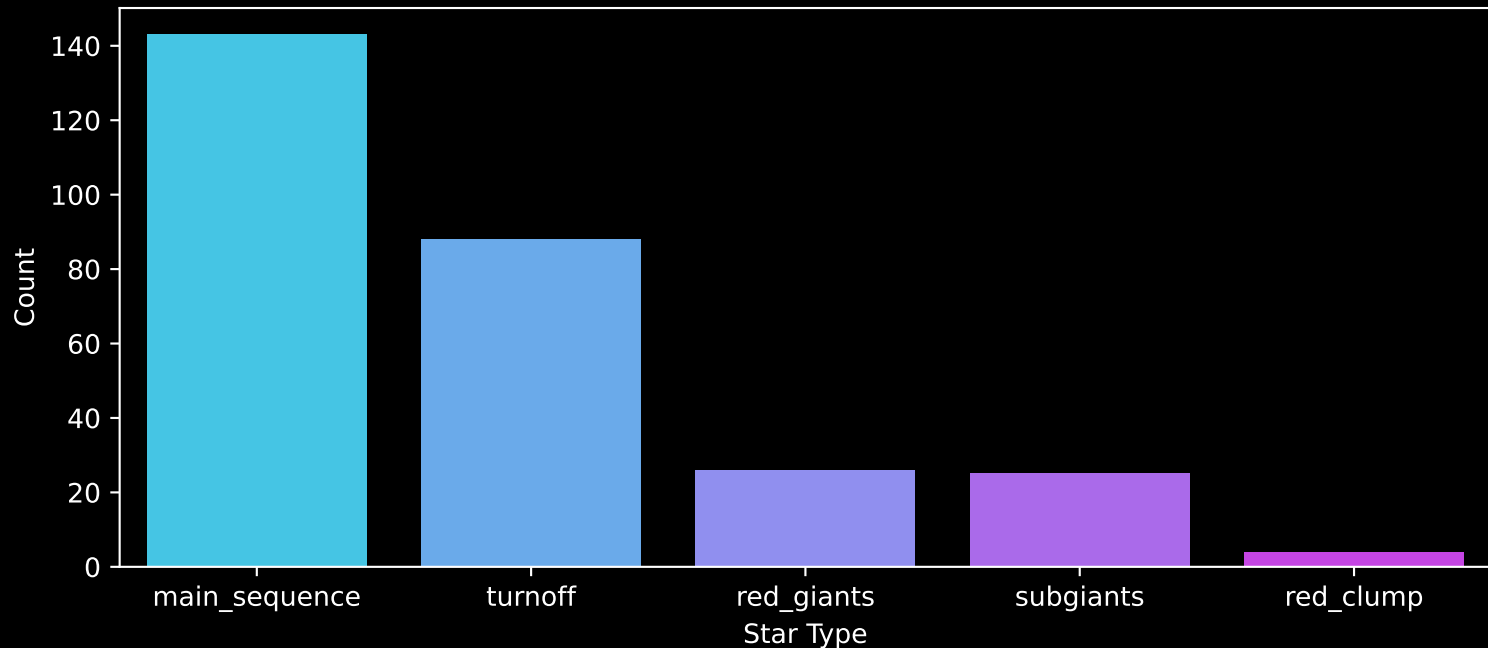
GALAH DR4 Field: [1599] Count plot of Star Type
